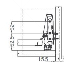
FA 面板重叠部分 Front board overlap
