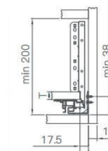
3. 箱体所需空间 Space requirements in cabinet
