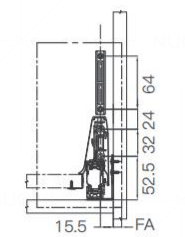
FA 面板重叠部分 Front board overlap
