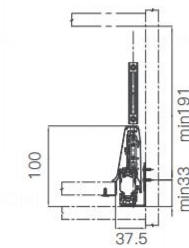
3. 箱体所需空间 Space requirements in cabinet
