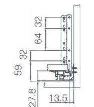
FA 面板重叠部分 Front board overlap
