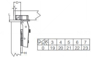
Full Overlay 直臂
