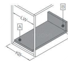
1. 箱体所需空间 Space requirements in cabinet
