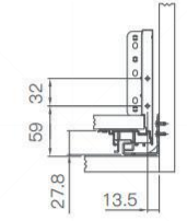
FA 面板重叠部分 Front board overlap
