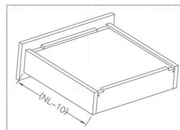
抽屉尺寸和钻孔(mm) Drawer size and drilling
