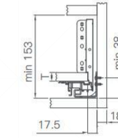
3. 箱体所需空间 Space requirements in cabinet
