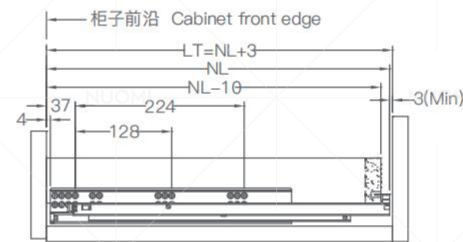
外置抽屉 Standard drawer
