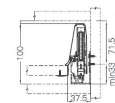
3. 箱体内部所需空间 Space requirements in cabinet
