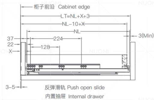
抽屉尺寸和钻孔(mm) Drawer size and drilling
