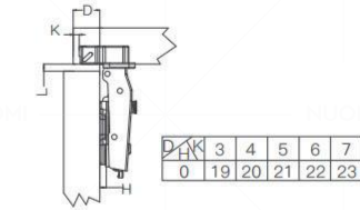
Full Overlay 直臂
